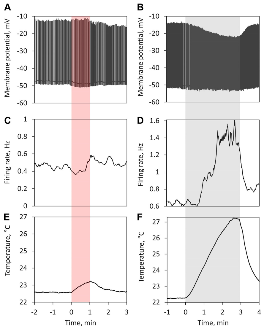
Fig. 2. Representative recordings of the electrophysiological activity in the Retzius cell (A and B), calculated firing rate (C and D), and bath temperature (E and F) during 60-s application of MMW irradiation ( 60 \text{ GHz} , 4 \text{ mW/cm}^2 ; A, C, E) and gradual bath heating (at a rate of 0.04^\circ\text{C/s} ; B, D, F). Calculation of the firing rate was based on the interspike intervals averaged for every 10 s. The shaded red area indicates the interval of MMW irradiation, and the shaded gray area indicates the interval of gradual bath heating.
