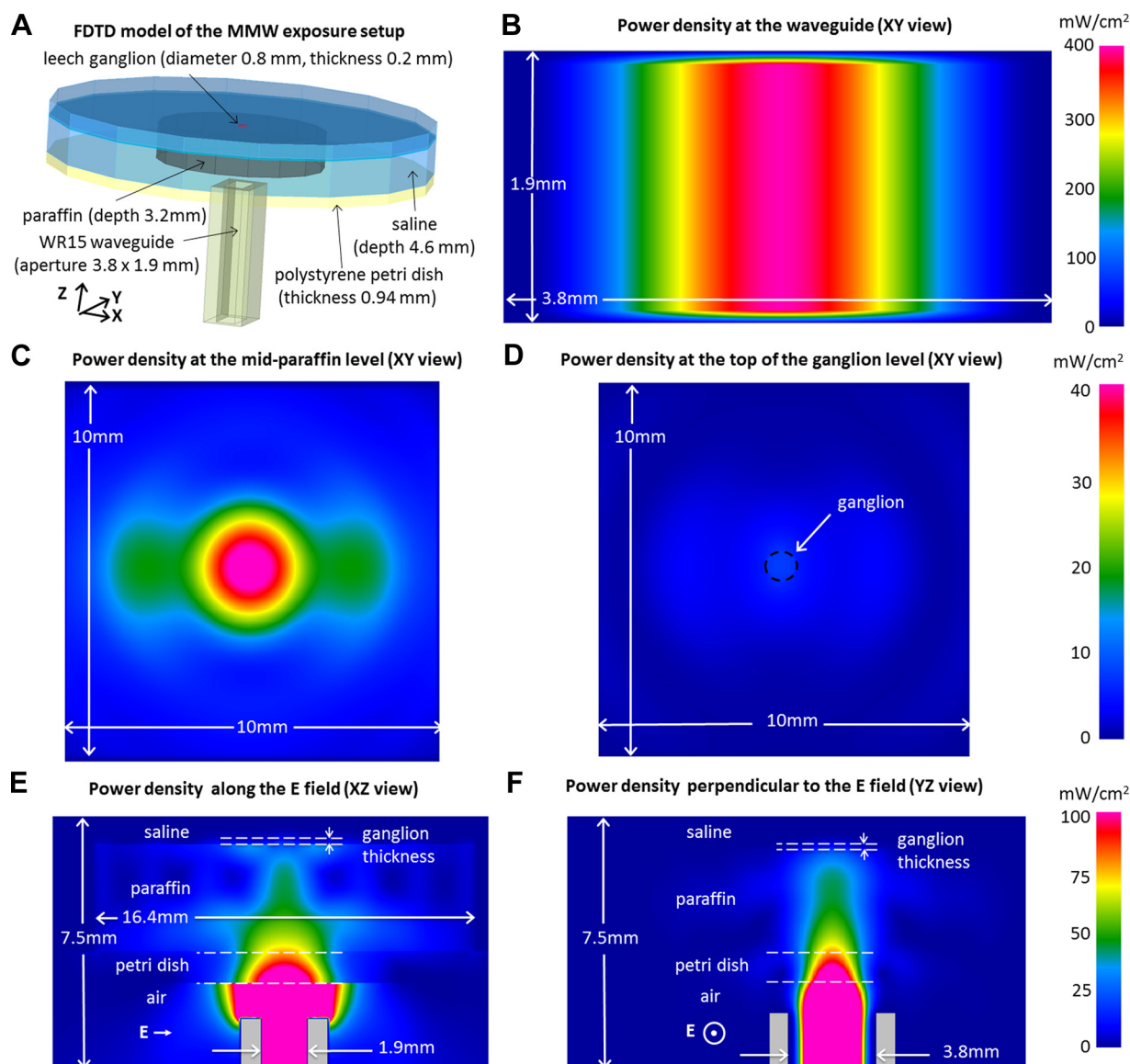
Fig. 1. A: 3-dimensional finite difference time domain (FDTD) model of the millimeter wave (MMW) exposure setup. B–D: simulated distribution of MMW power density in several cross sections through the FDTD model taken either along (B, E, and F) or perpendicular to the MMW path at the paraffin level (C) and at the top-of-the-ganglion level (D). Linear pseudocolor power density scales are provided at right for each row of cross sections. The FDTD simulations were performed at an injected MMW power level in the waveguide of 16 mW, corresponding to an incident power density (IPD) of 4 mW/cm 2 at the top-of-the-ganglion level.
