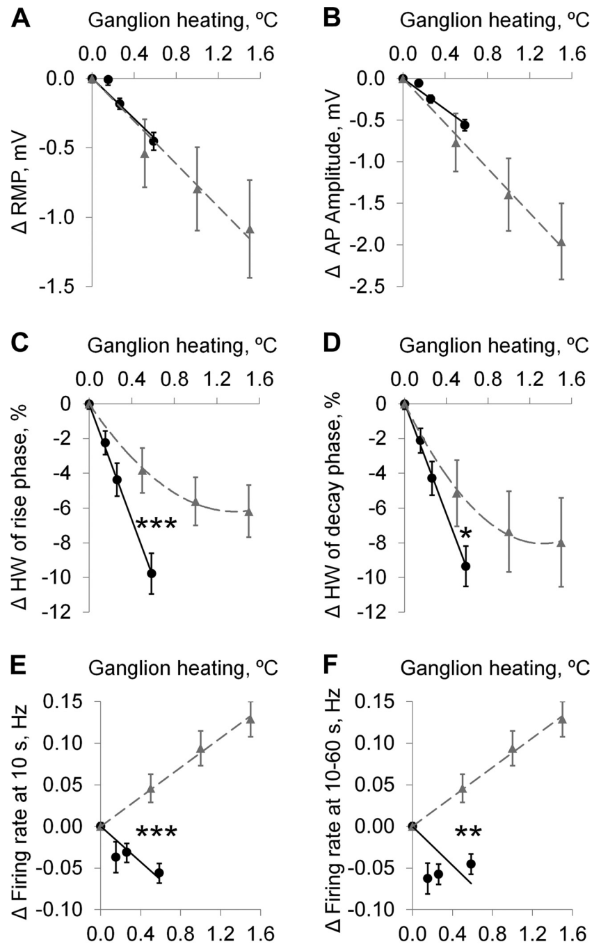
Fig. 5. Comparison of the heating effects induced by MMW irradiation at 3 IPD levels (circles) and by gradual bath heating (triangles) on changes in the following action potential (AP) parameters in the Retzius cells: maximal change in resting membrane potential ( \Delta RMP; A ), maximal change in AP amplitude ( \Delta AP amplitude; B ), maximal change in half-width ( \Delta HW) of the rise phase ( C ), maximal \Delta HW of the decay phase ( D ), \Delta firing rate at 10 s after initiation of MMW exposure ( E ), and average \Delta firing rate at 10–60 s after initiation of MMW exposure ( F ). Data are means \pm SE. * P < 0.05 ; ** P < 0.01 ; *** P < 0.001 for 1-tailed t -test comparing the MMW and bath heating effects at the heating level of 0.6°C. Linear regression lines are shown for MMW irradiation (solid) and gradual bath heating (dashed).
